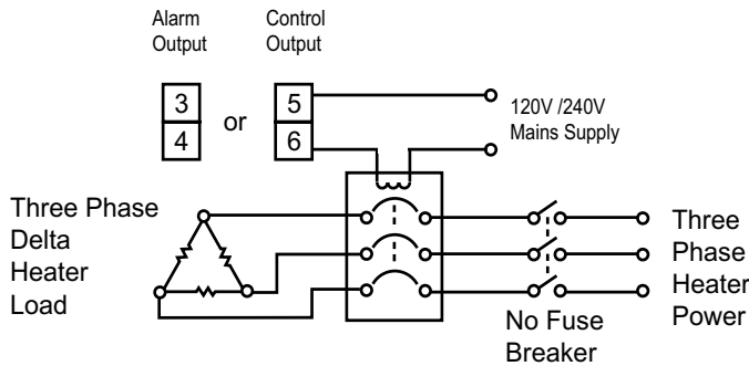
Fig. 4.10 Contactor drive Connections
