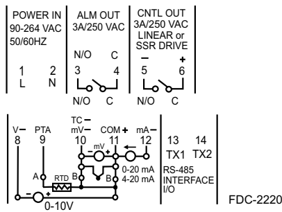
Fig. 4.3 Rear Terminal Connections
