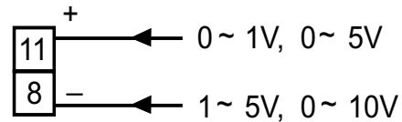
Fig. 4.7 Linear Voltage Input Connections
