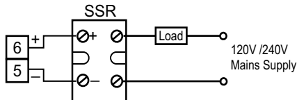
Fig. 4.11 SSR Drive Connections
