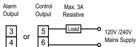
Fig. 4.9 Relay Direct Drive Connections
