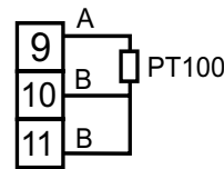
Fig. 4.6 RTD Input Connections
